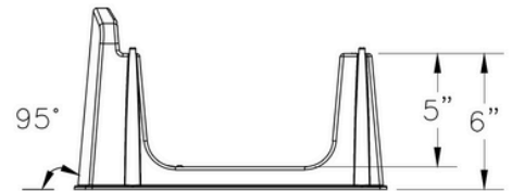
SIDE VIEW WITHOUT SIDE RAILS
