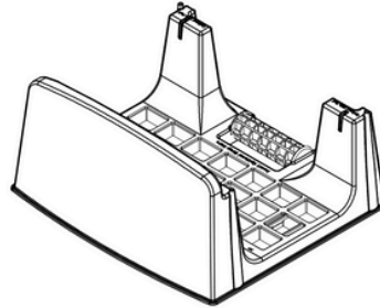
ISO VIEW WITHOUT SIDE RAILS
